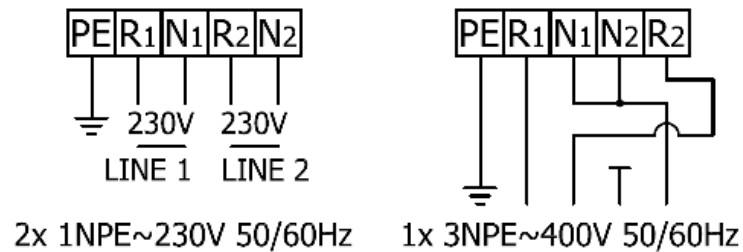
Figure 19. Optional Connections
