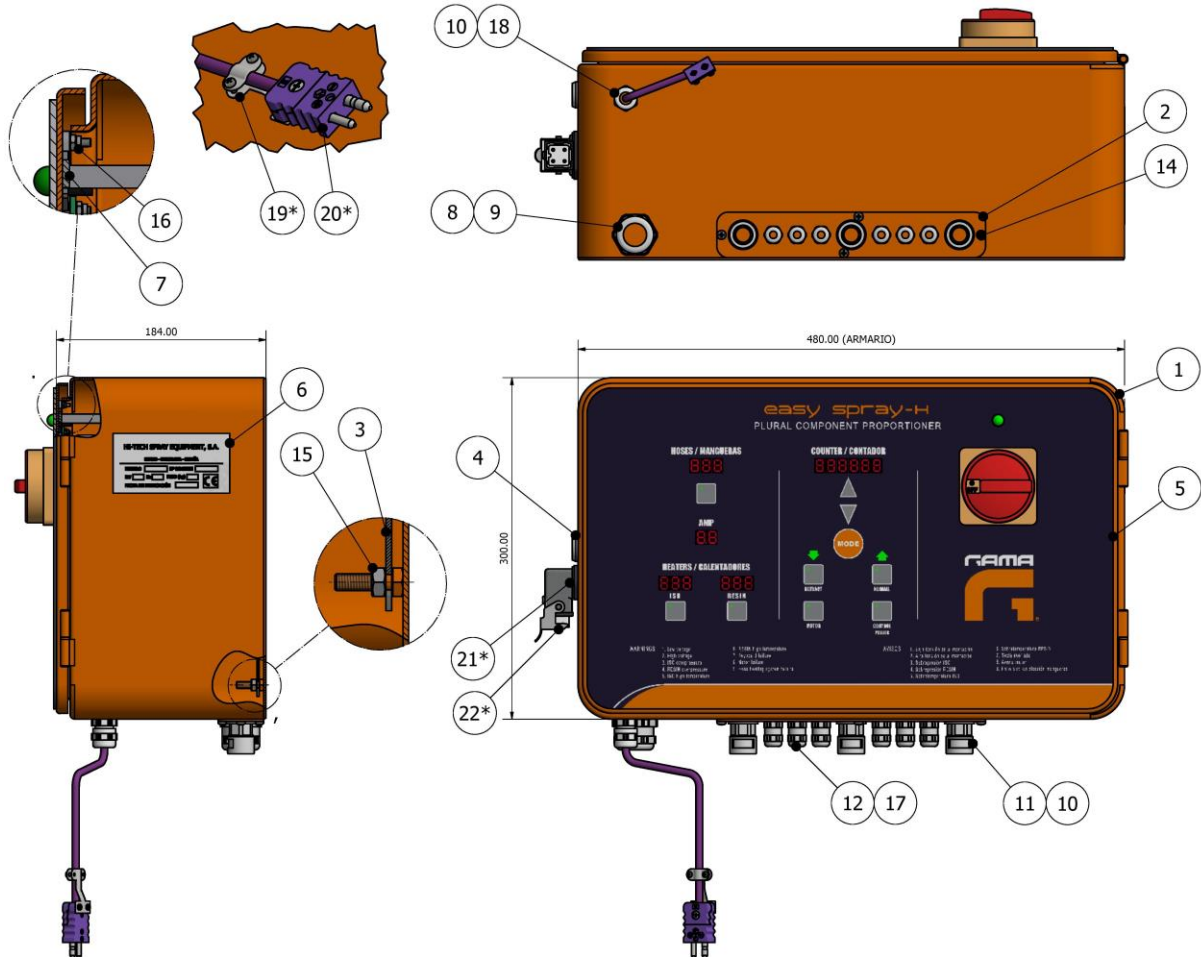
Figure 2. Electrical console for Easy Spray - H
