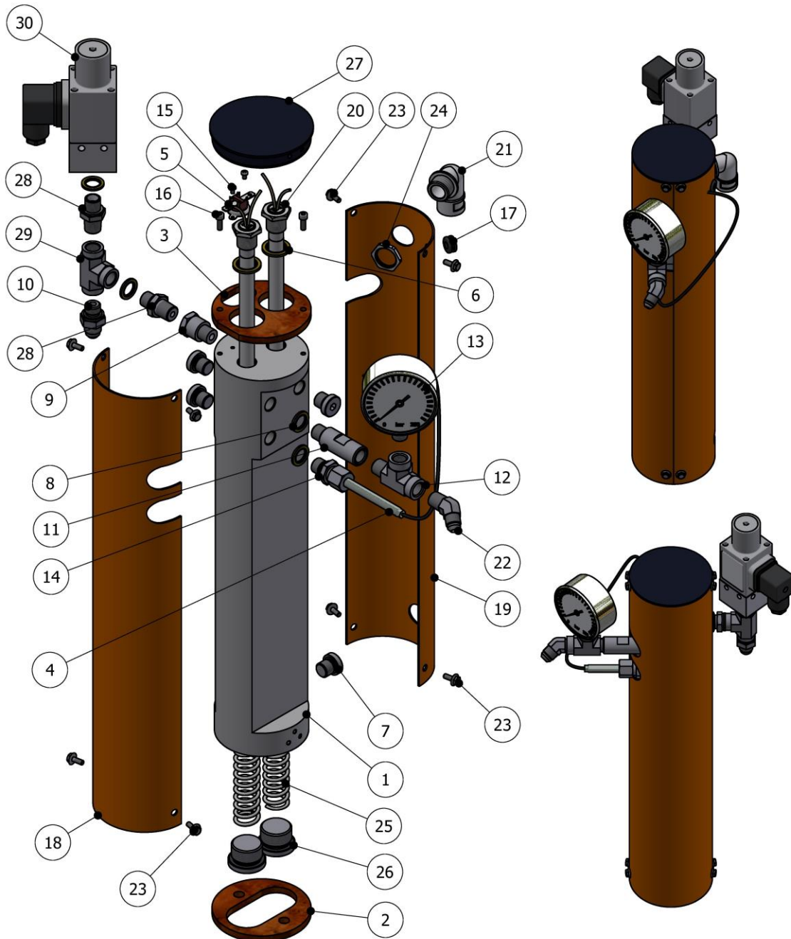
Figure 8. Primary heater
