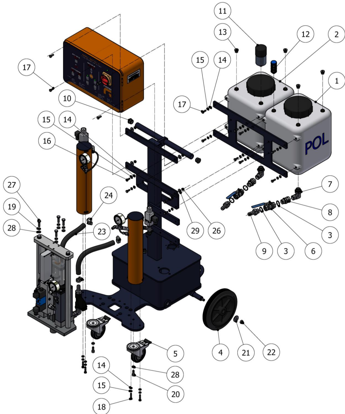
Figure 4. Framework components
