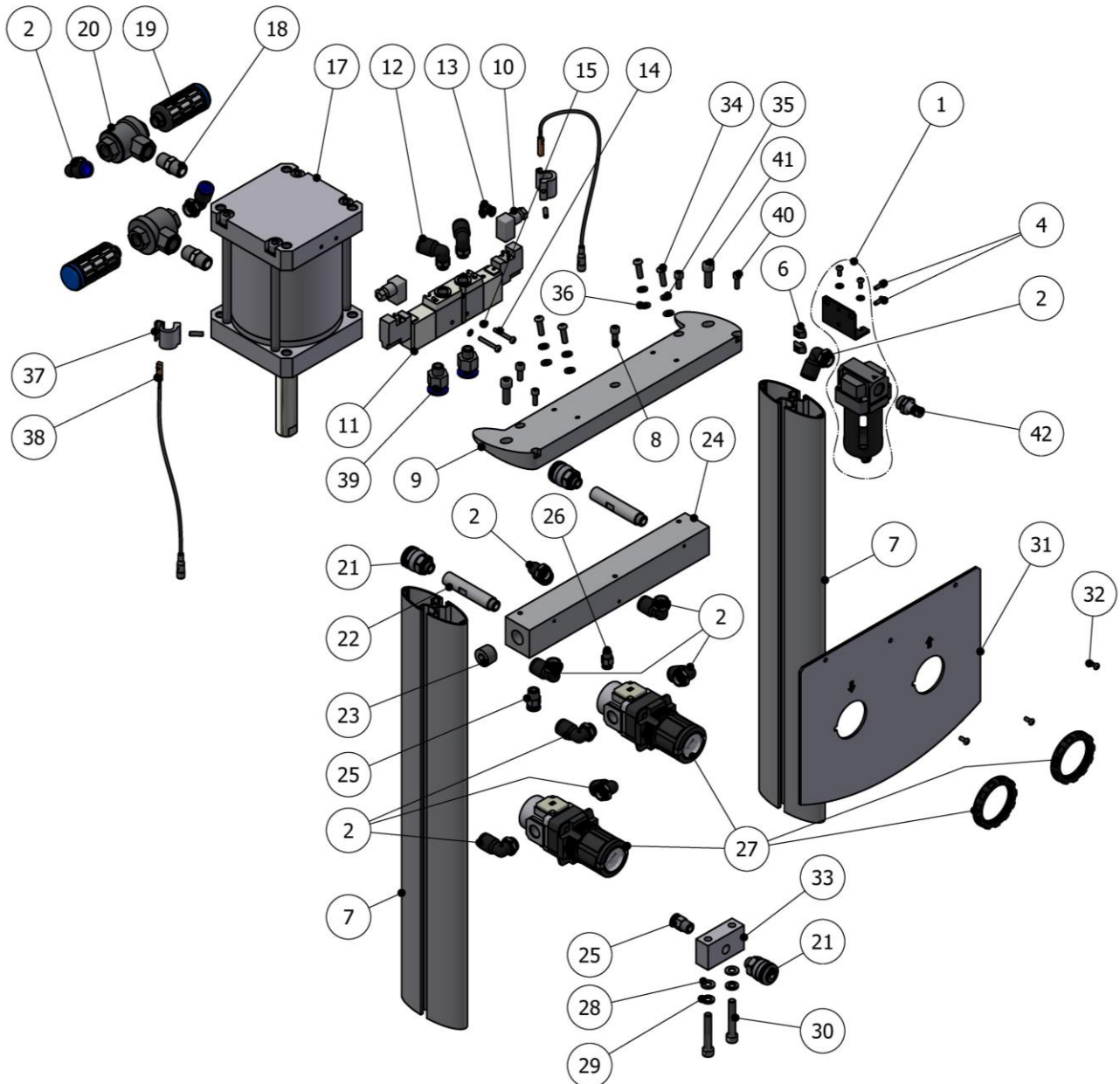
Figure 10. Air Control Assembly, Exploded View
