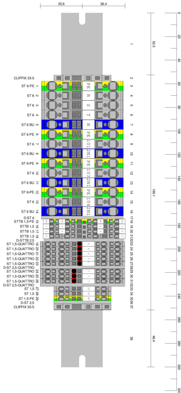
Figure 24. Electrical Distribution 3NPE~400V 50/60 Hz, Sheet 8 of 9
